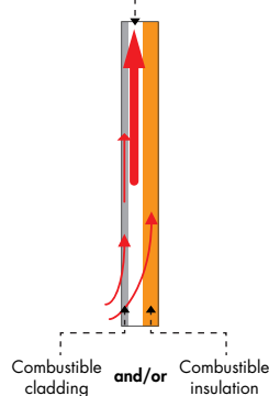
Chimney effect, increasing the speed of fire spread through the air cavity
