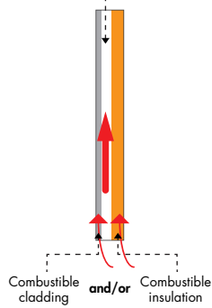
Chimney effect, increasing the speed of fire spread through the air cavity
