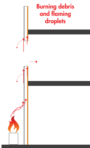
Chimney effect, increasing the speed of fire spread through the air cavity
