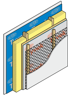
Fig. 7 Timber Frame Cement render on lathe
