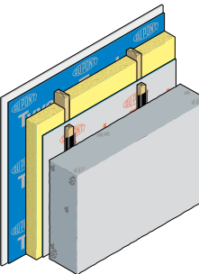
Fig. 10 Masonry wall Internal insulation upgrade
