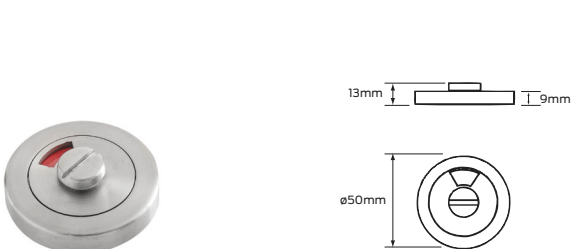
Indicating emergency release #7014
