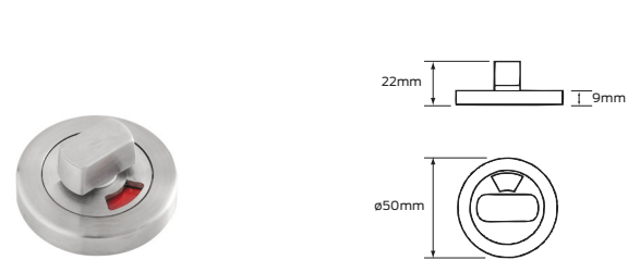
Indicating turn #7013
