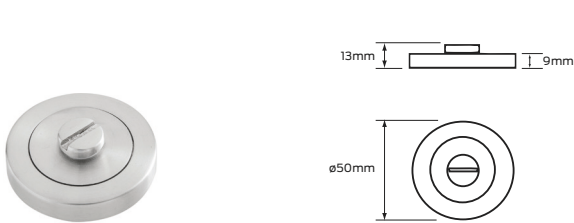
Emergency release #7009
