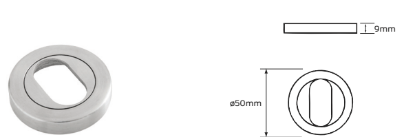
Cylinder #7008
