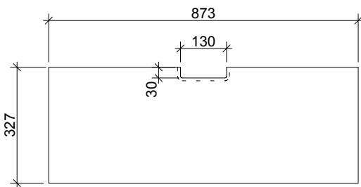
DRAWER FRONT
