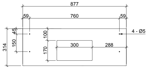
FRAME REAR
