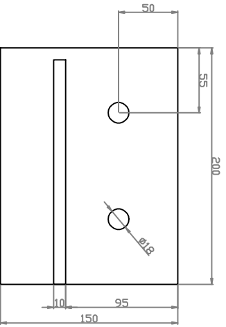
Safety Side Mounted Clevis Plan Scale 1:1
