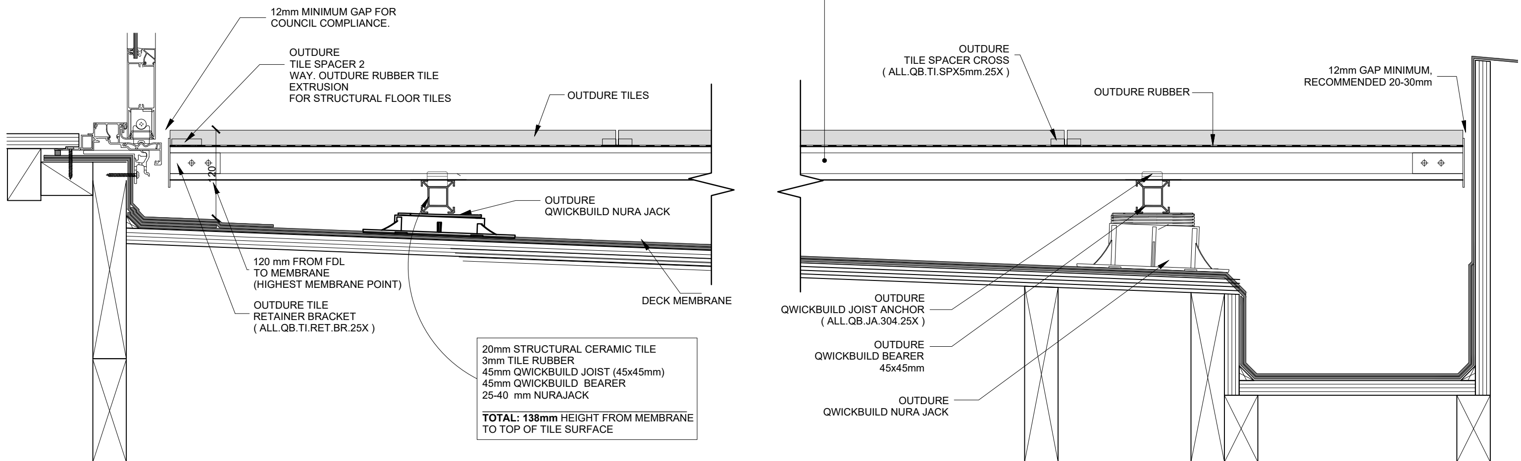
1 QB -T3. 120mm LOW HEIGHT TILE DETAIL SCALE 1:5
