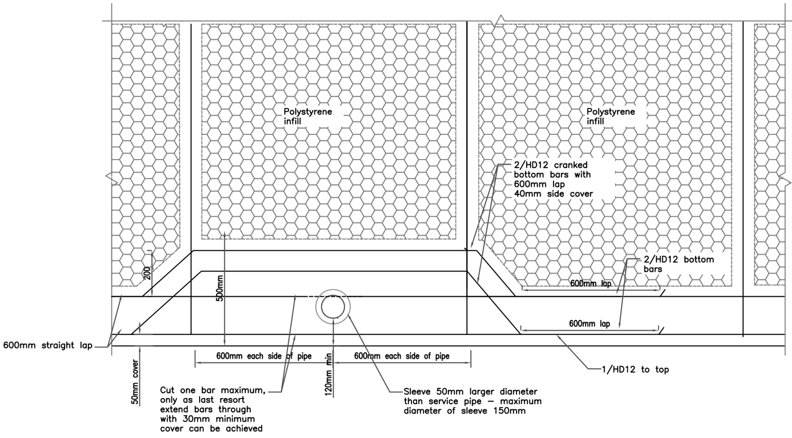
TYPICAL SERVICES THROUGH PERIMETER FOOTING
