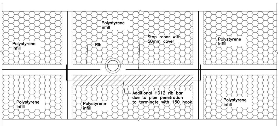
TYPICAL SERVICES THROUGH RIBS
