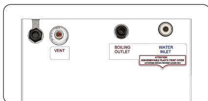
Fig 5. Boiling Only model: Connection viewed from the top
