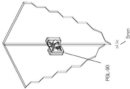
PGL-90 Glass to Glass Lock
