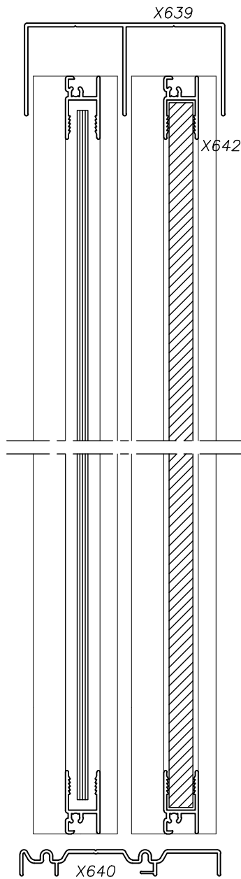
SECTION AA
