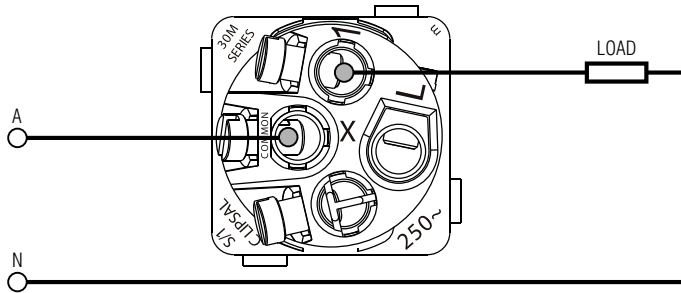
One-Way Switching
