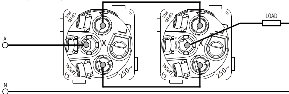
Two-Way Switching
