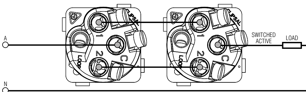
Two-Way Switching
