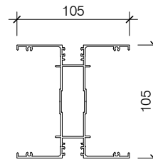
PAS024 105 CORNER POST
