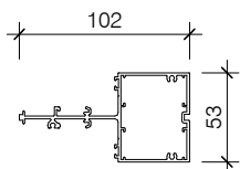
PAS021 105 GLAZING SILL/TRANSOM
