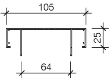
PAS010/R 64mm CAPPING HEAD/FRA
