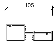
PAS021/A 105 GLAZING SILL/TRANSOM
