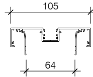
PAS014 105 PLASTERBOARD POCKET CAPPING/FRA
