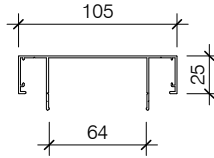
PAS010 105 HEAD/SILL TRACK
