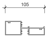
PAS021/A 105 GLAZING SILL/TRANSOM
