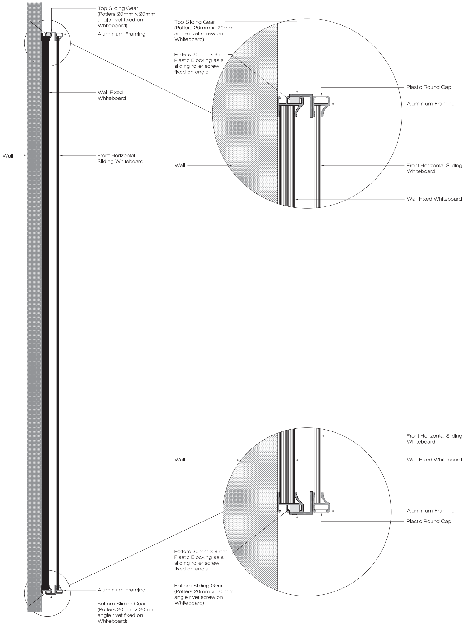
Cross section F - F
