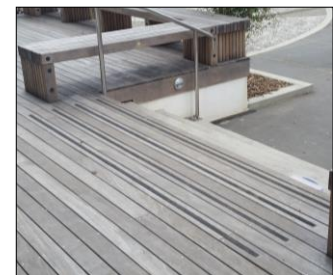
SlipFree insert in Vitex Decking - Muritai School, Wellington
