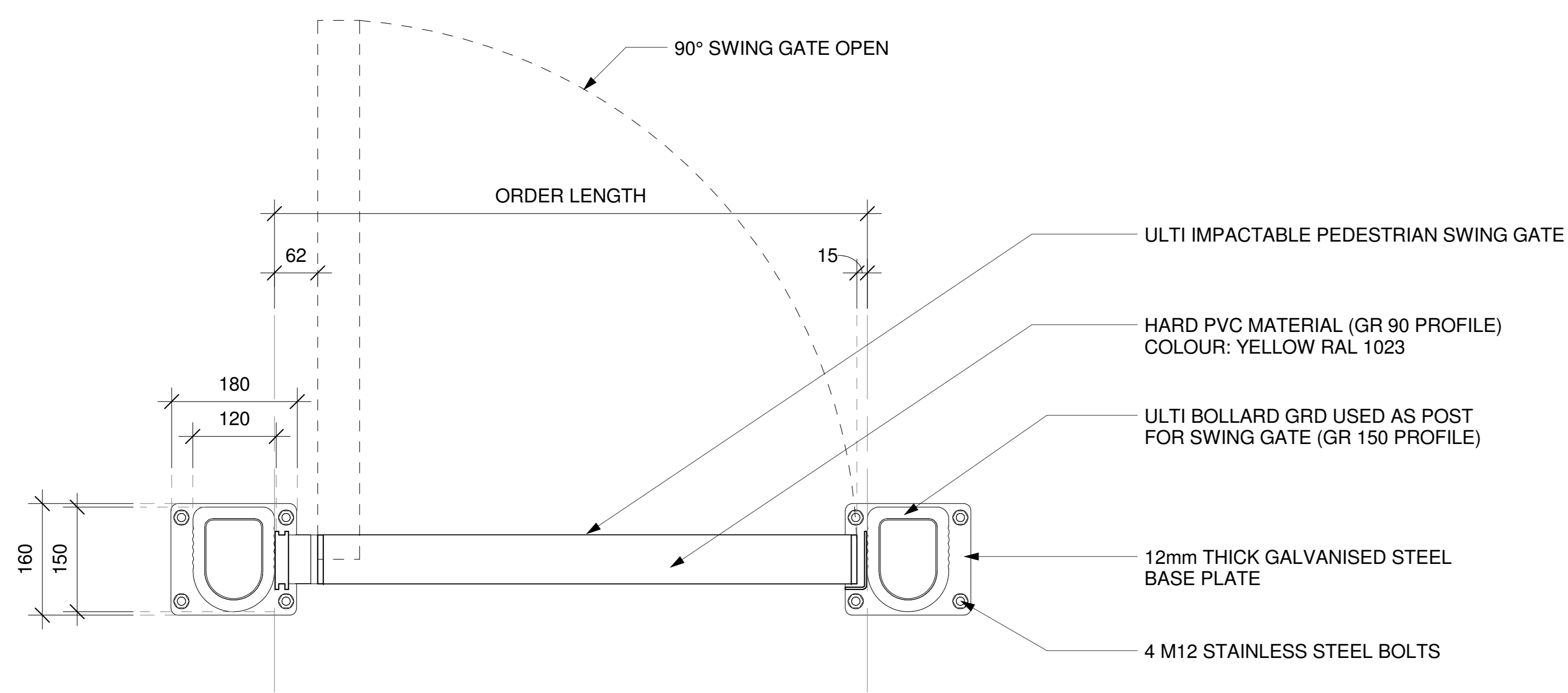
1 PLAN VIEW - DP 150 SCALE: 1:5 MTS.
