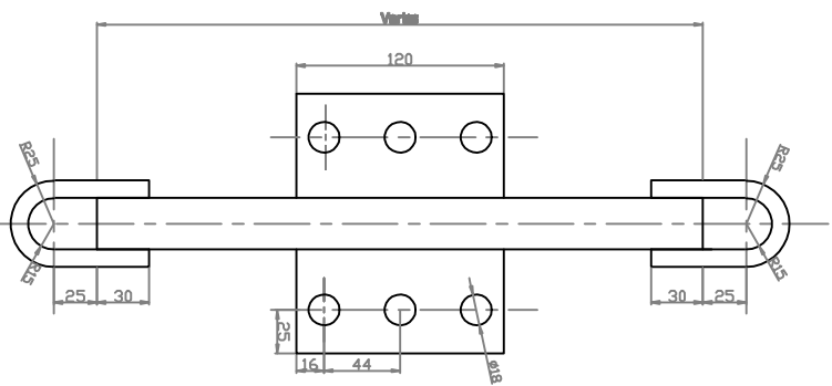
DE013 Roof Anchor Plan Scale 1:1
