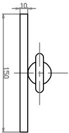
Elevation A Scale 1:1
