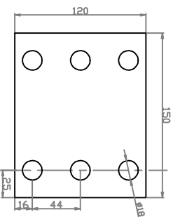
Rear plate Plan Scale 1:1
